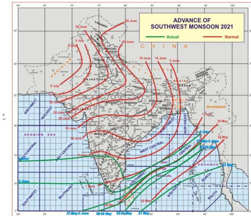
Fig 1: Northern Limit of the southwest Monsoon 2021 as on 4 June 2021
