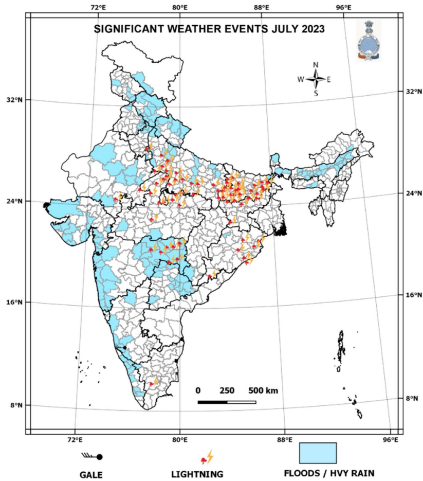
Fig. 11: Significant weather events during July 2023 (Based on real-time media report)-
