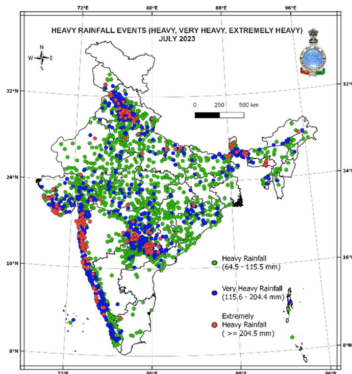
Fig 5: The location of occurrence of heavy rainfall events in the month of July 2023.
