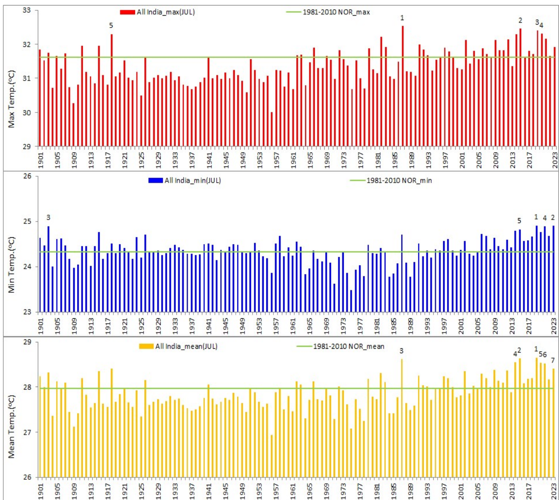
Fig 8: Time series of monthly average maximum, average minimum and mean temperature over the country as a whole for the month of July 1901-2023.
