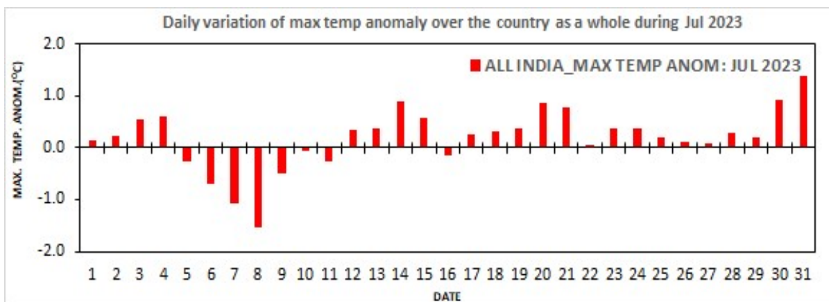
Fig 7(a): Daily variation of maximum temperature anomaly over the country as a whole for July 2023.
