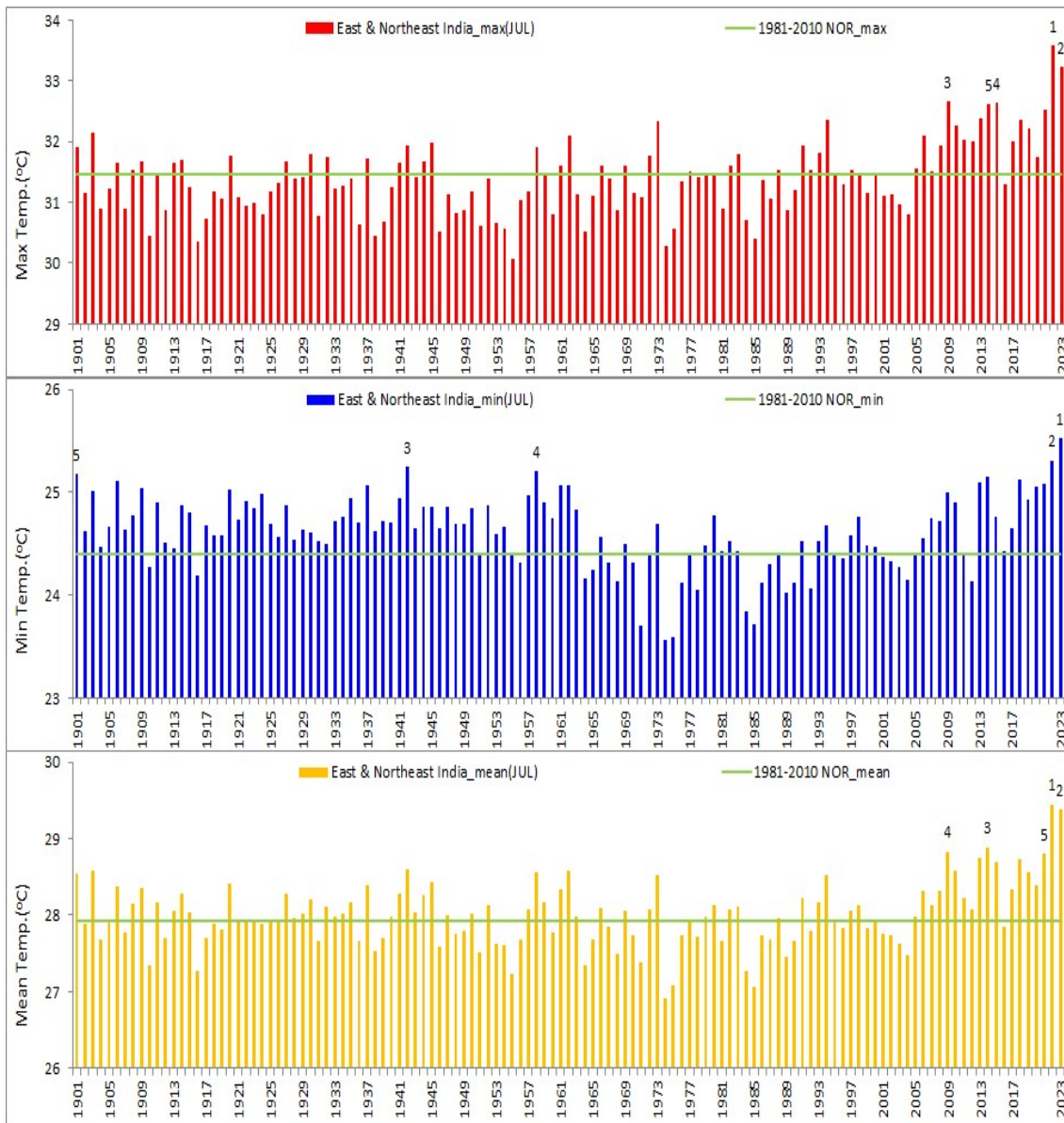
Fig 9: Time series of monthly average maximum, average minimum and mean temperature over East & Northeast India for the month of July 1901-2023.
