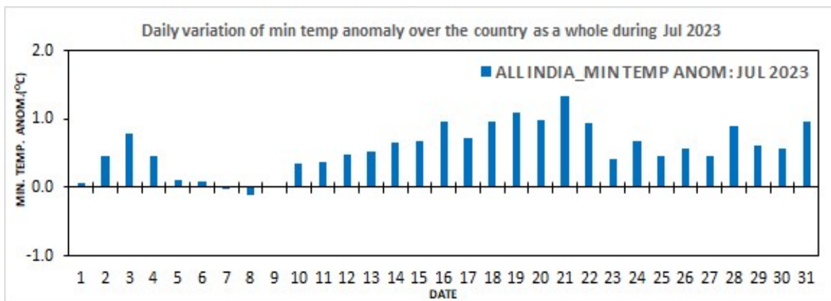
Fig 7(b): Daily variation of minimum temperature anomaly over the country as a whole for July 2023.
